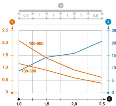
Load diagram, cable tray, type RKS-Magic 60
